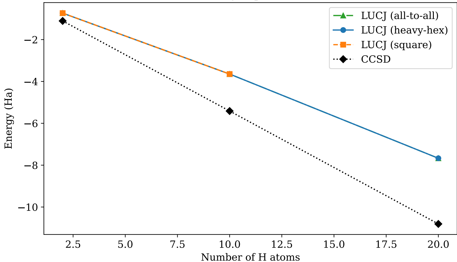
H chain: order--1 LUCJ expectation value vs CCSD
