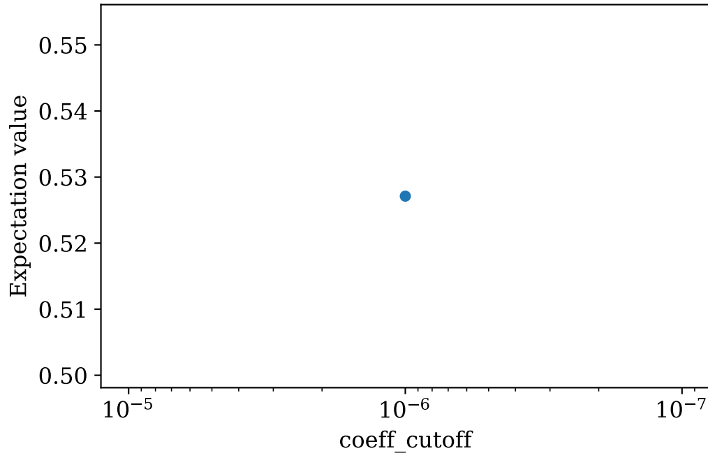
Z-string (w=2), damping=0.001
