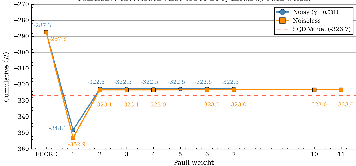
Cumulative expectation value of FeS LUCJ ansatz by Pauli weight
