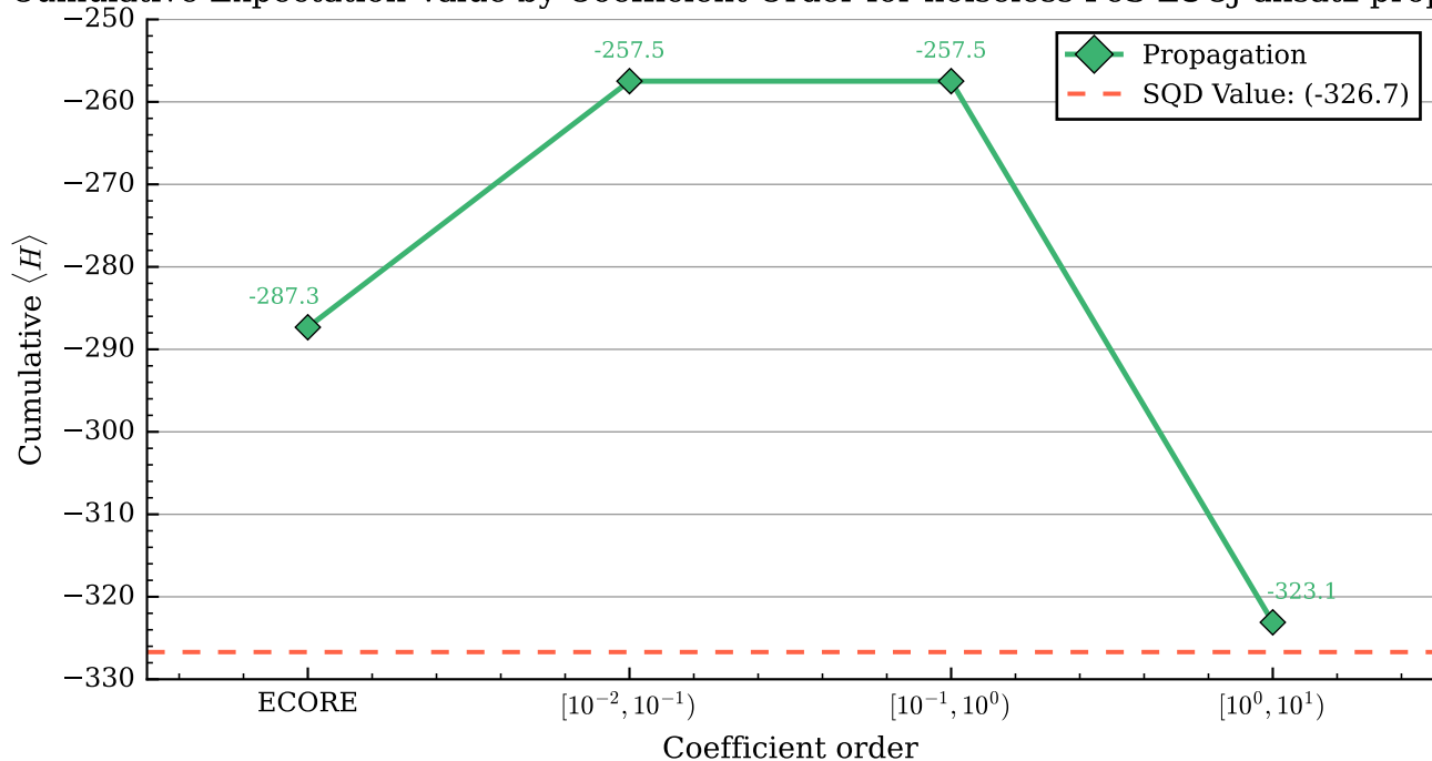
Cumulative Expectation Value by Coefficient Order for noiseless FeS LUCJ ansatz propagation
