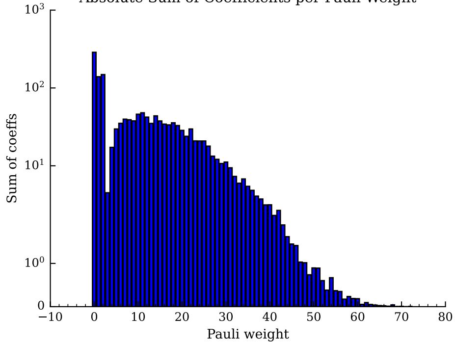
Absolute Sum of Coefficients per Pauli Weight
