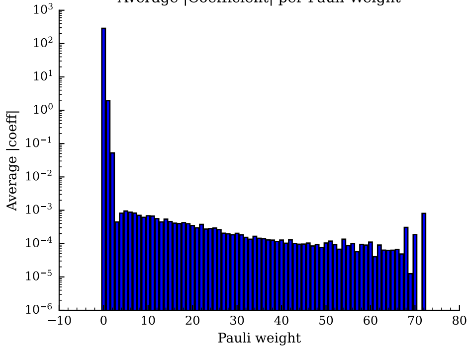
Average |Coefficient| per Pauli Weight
