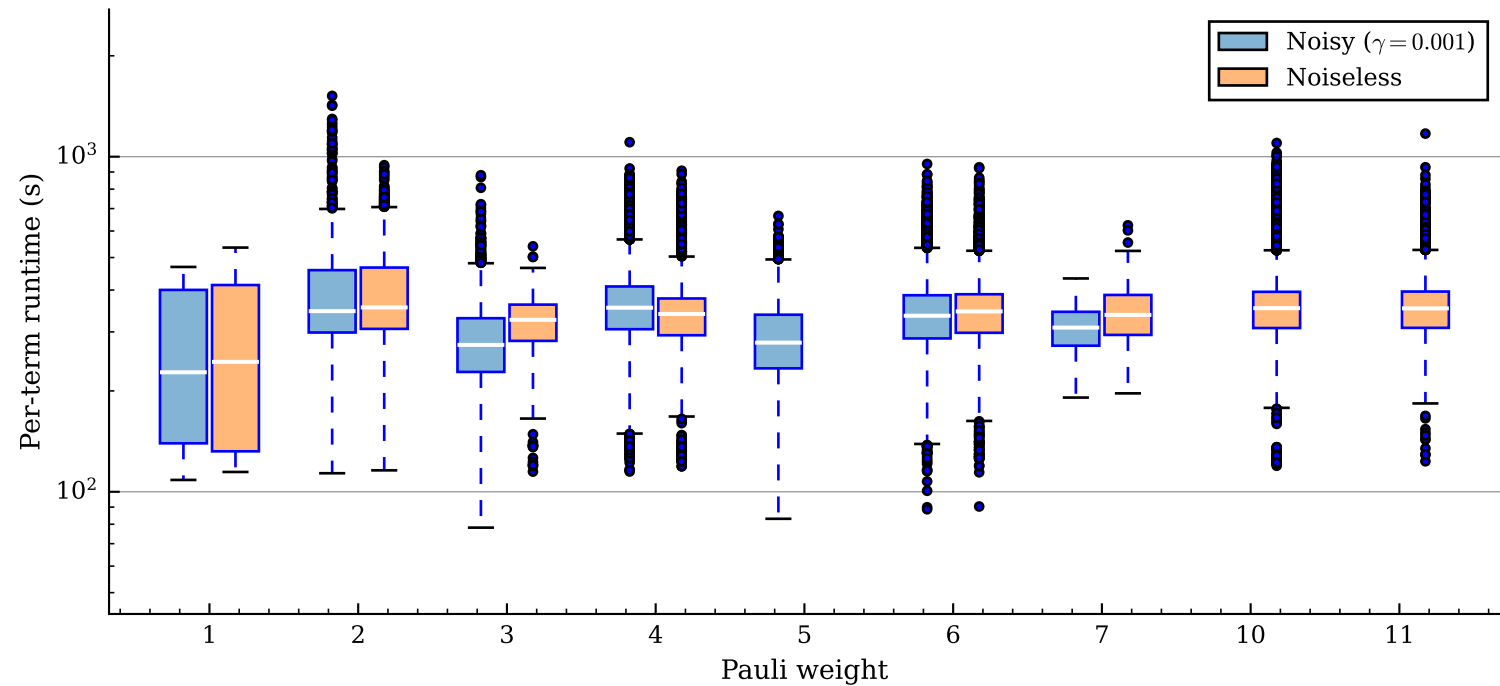
Per-term wall-clock runtime of FeS LUCJ ansatz propagation by Pauli weight
