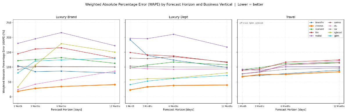
Figure C4. Weighted Absolute Percentage Error (WAPE) by forecast horizon, shown separately for each business vertical.
