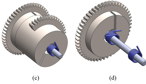
Figure 7. The Idle-Stroke Gear.
