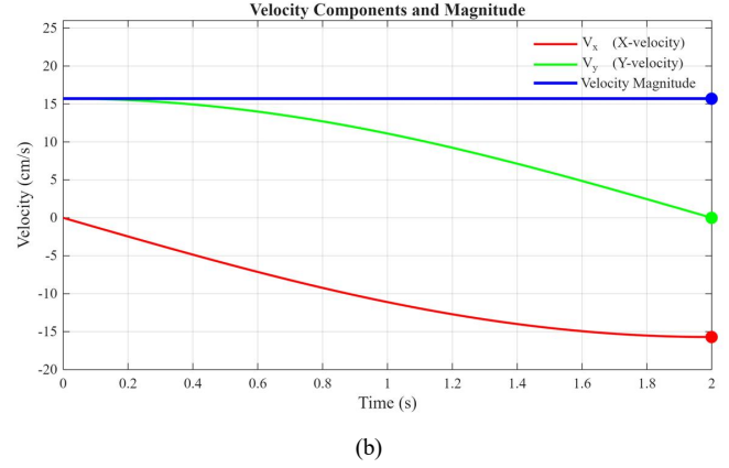
Figure 10. Analysis of trajectory and velocity of C : (a) Parallelogram Mechanism Motion Analysis, (b) Velocity Components and Magnitude.
