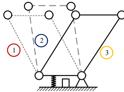
Figure 2. Parallelogram Linkage Mechanism.
