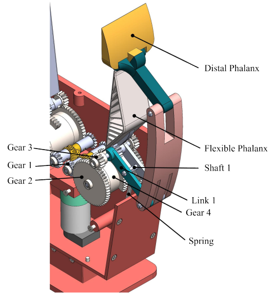
Figure 6. The Design of the Biocrest finger.
