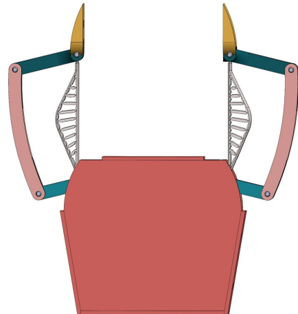
Figure 1. The BioCrest gripper.
