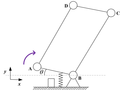
Figure 9. The planar parallelogram mechanism.
