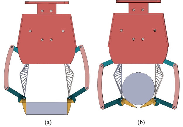
Figure 8. Two grasping modes of the Biocrest gripper. (a) Linear parallel pinching for precision grasp; (b) Self-adaptive grasping for power grasp.
