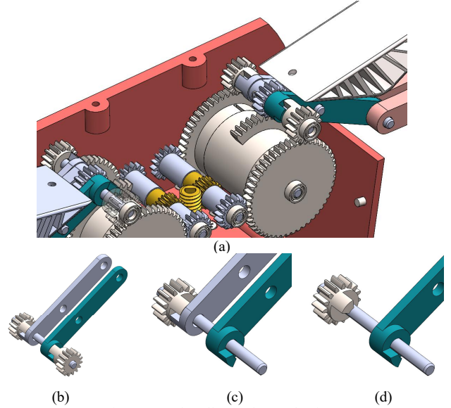
Figure 3. The Idle-Stroke mechanism.
