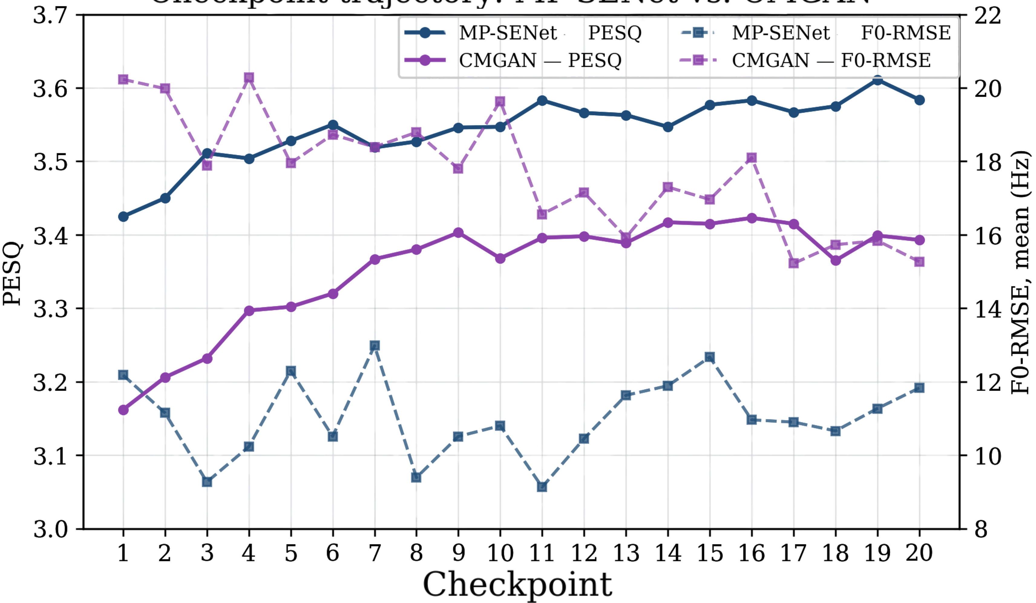
Checkpoint trajectory: MP-SENet vs. CMGAN
