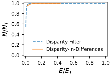
World Trade Network
