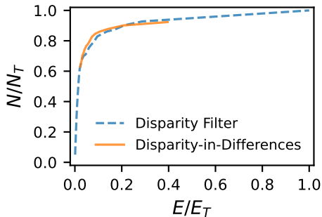
U.S. Airport Network
