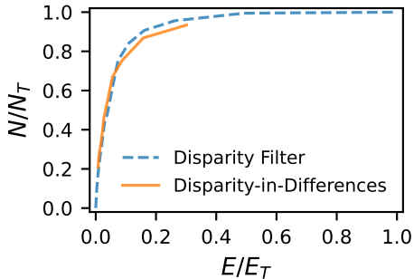
Enron Email Network
