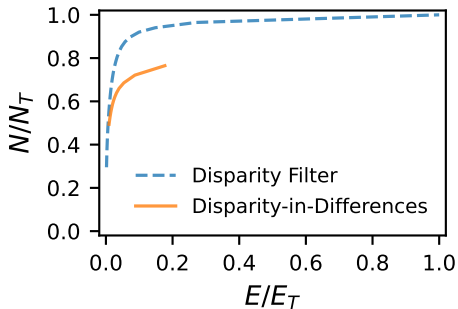
Journal Citation Network
