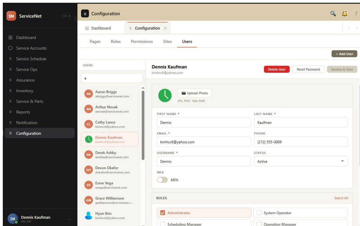
Configuration — Users.
