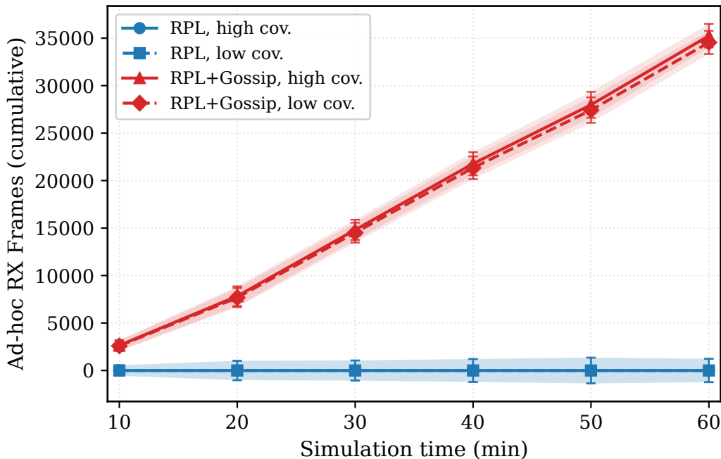
Ad-hoc RX Frames - 30 nodes, random
