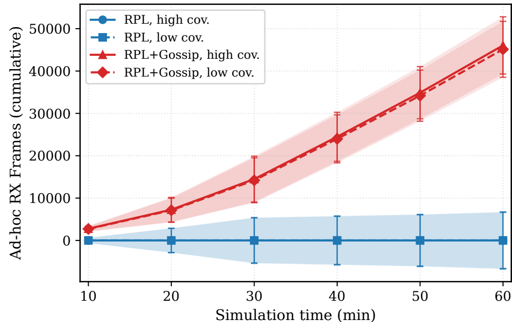
Ad-hoc RX Frames - 40 nodes, grid
