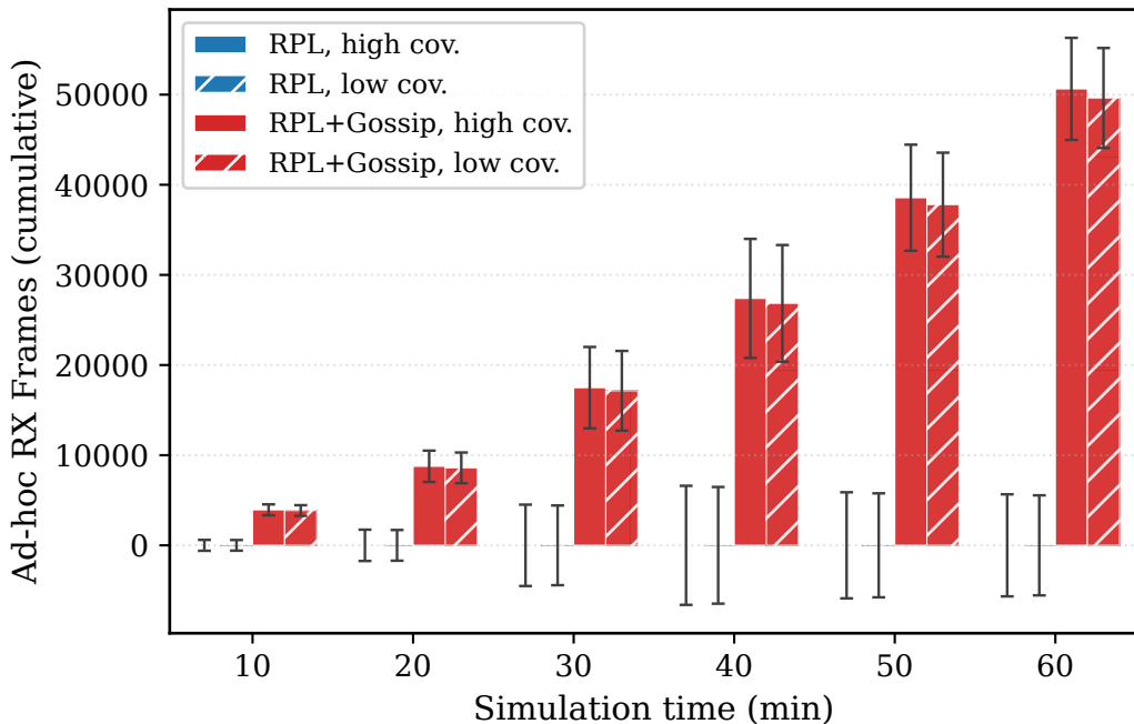
Ad-hoc RX Frames - 40 nodes, random
