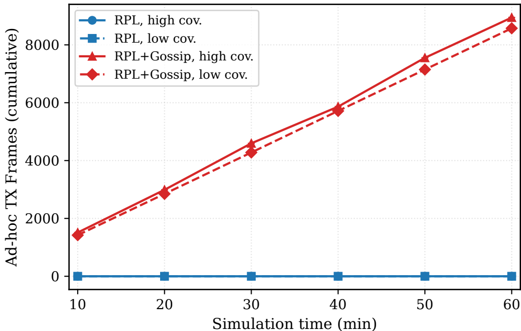
Ad-hoc TX Frames - 30 nodes, grid
