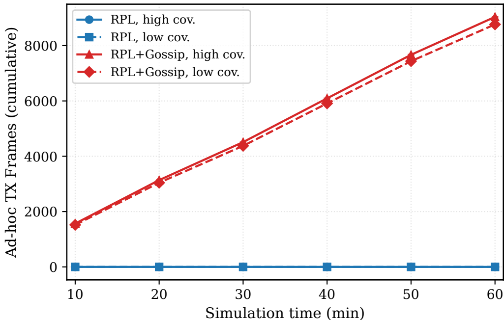
Ad-hoc TX Frames - 30 nodes, random
