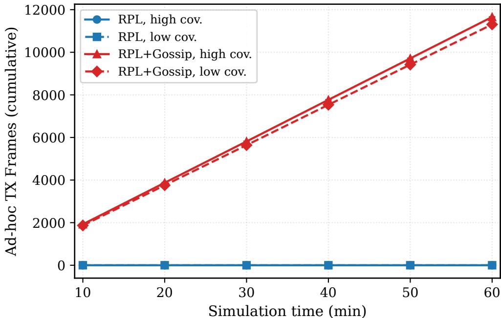
Ad-hoc TX Frames - 40 nodes, grid
