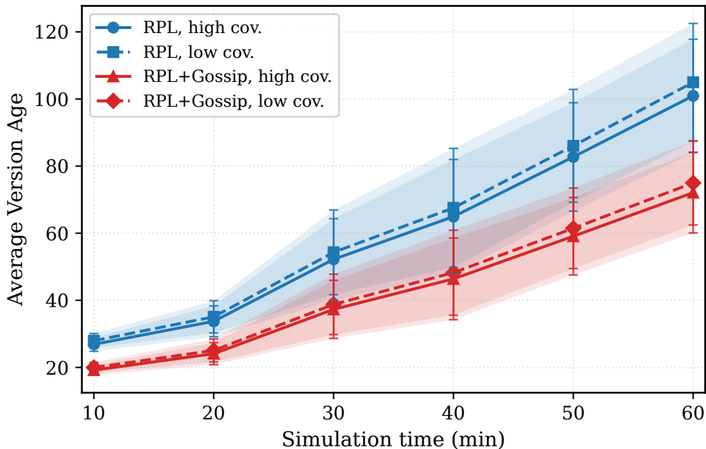
Average Version Age - 40 nodes, random
