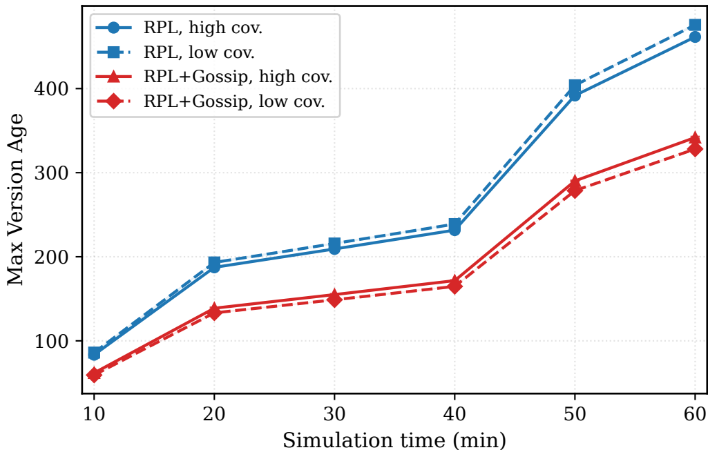
Coverage (Max Version Age) - 30 nodes, random
