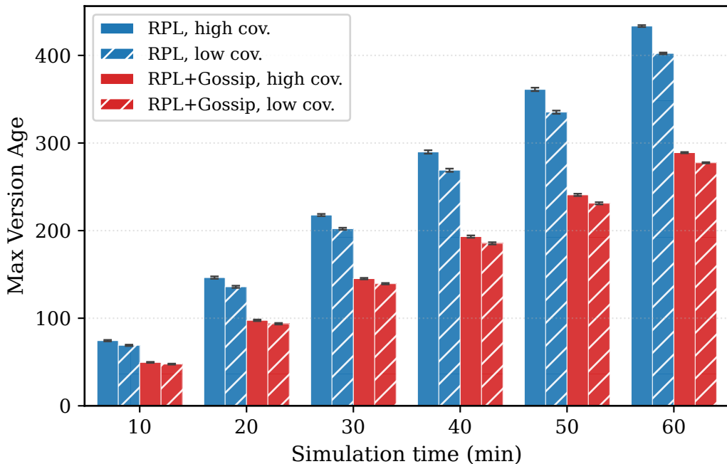
Coverage (Max Version Age) - 40 nodes, grid
