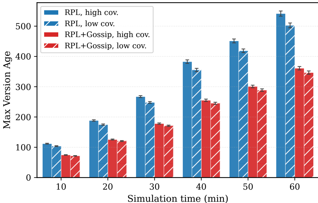
Coverage (Max Version Age) - 40 nodes, random
