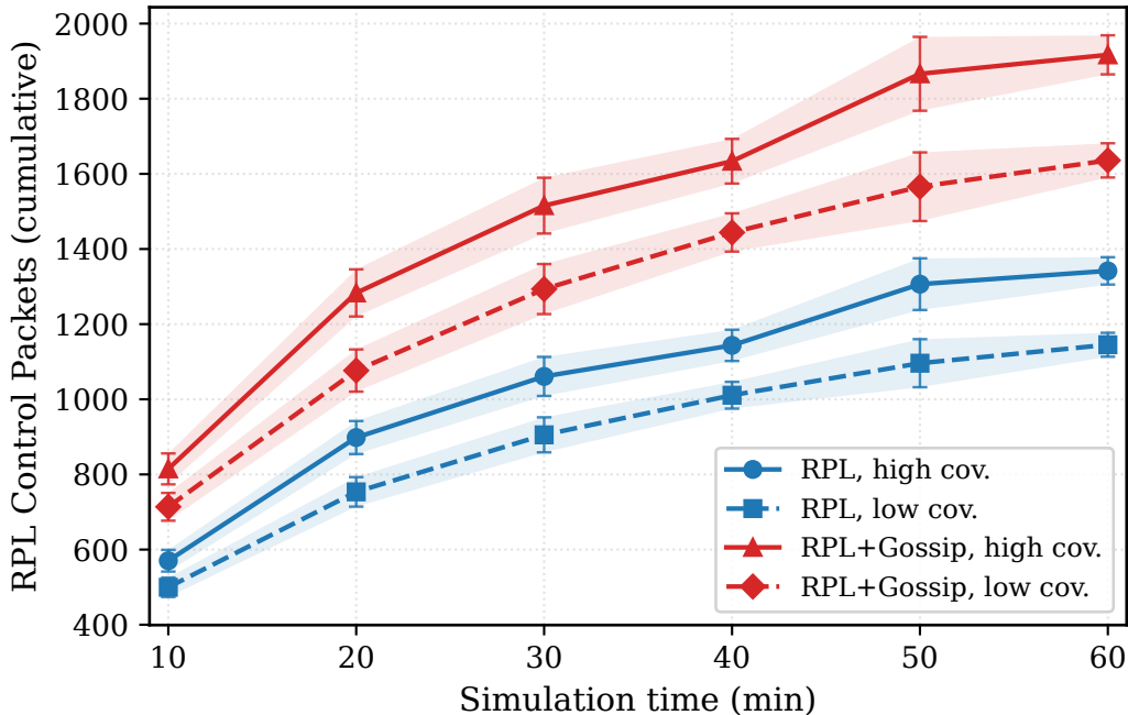
Control Overhead (DIO+DIS+DAO) - 30 nodes, grid
