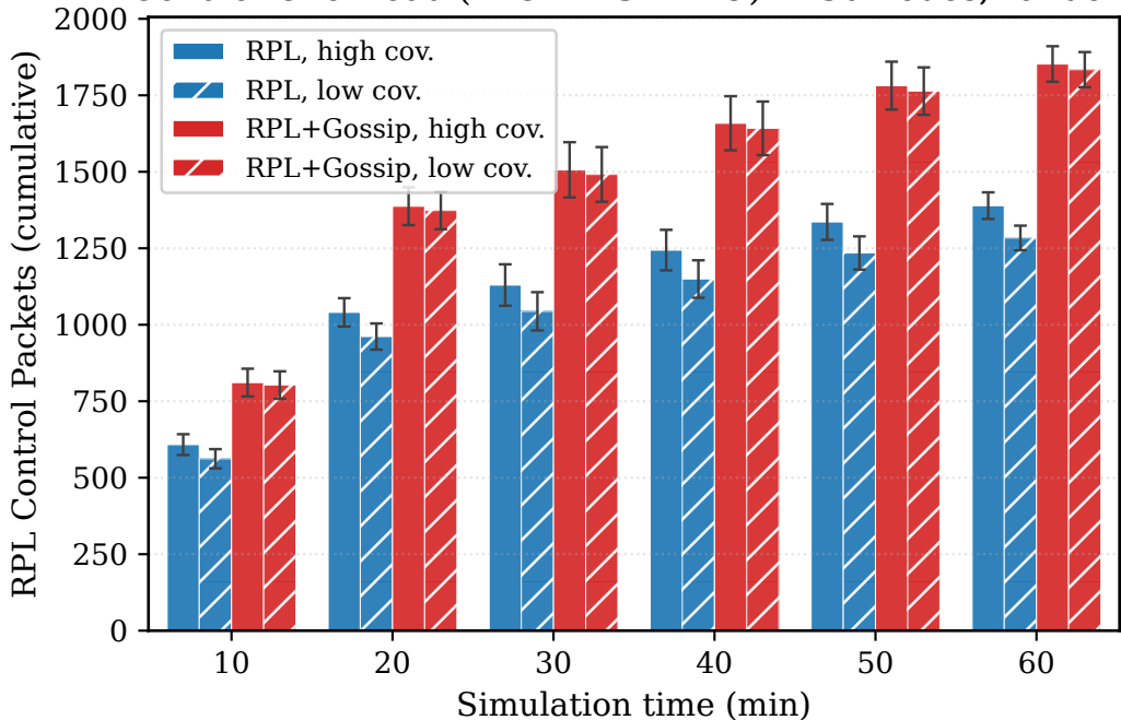
Control Overhead (DIO+DIS+DAO) - 30 nodes, random
