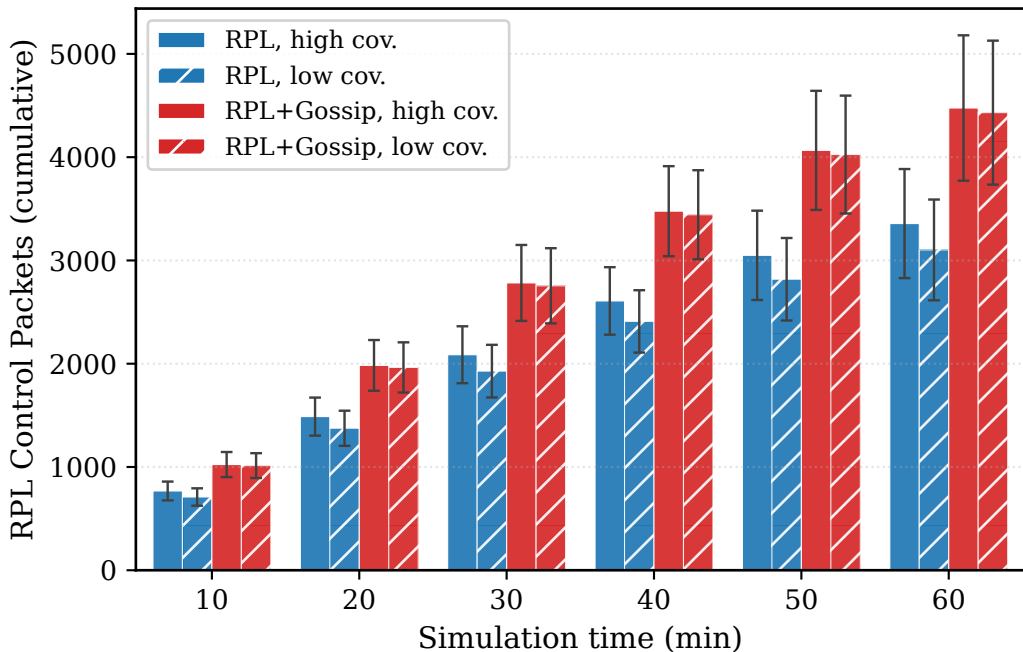
Control Overhead (DIO+DIS+DAO) - 40 nodes, grid
