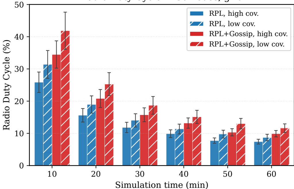
Radio Duty Cycle - 30 nodes, grid
