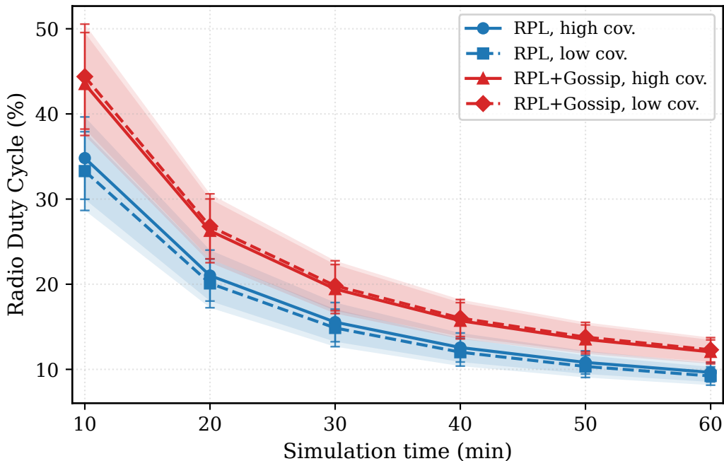
Radio Duty Cycle - 30 nodes, random
