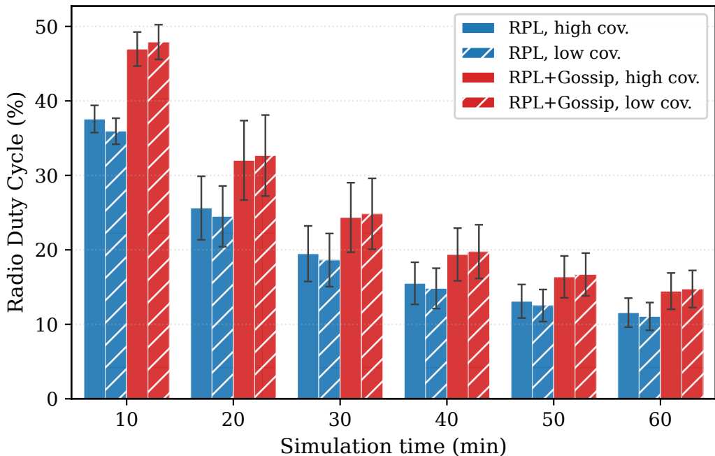
Radio Duty Cycle - 40 nodes, grid
