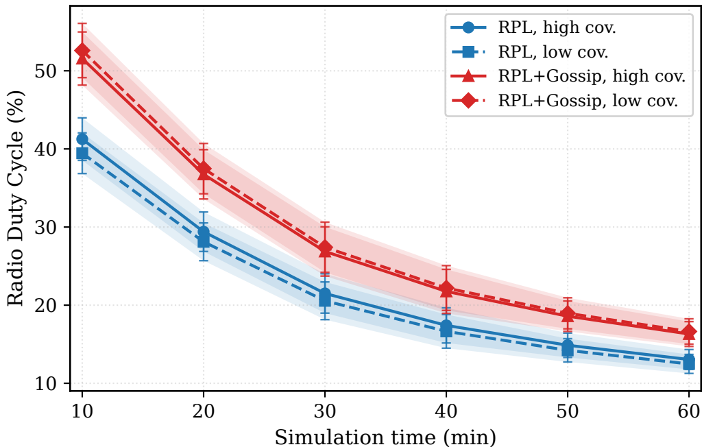
Radio Duty Cycle - 40 nodes, random
