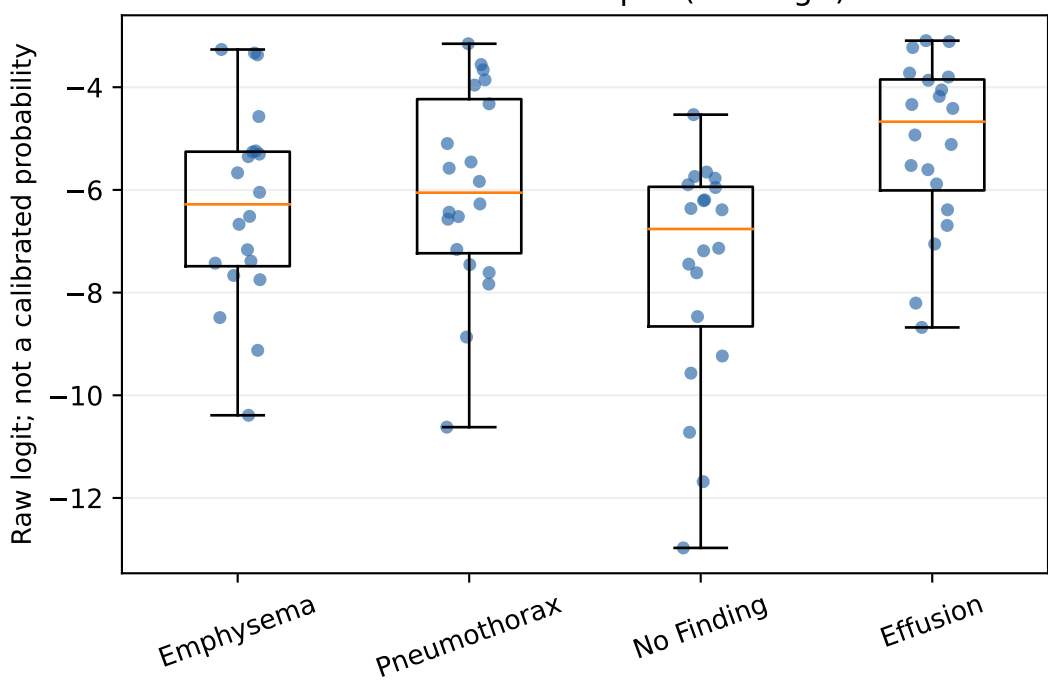
Pneumothorax output (raw logit)
