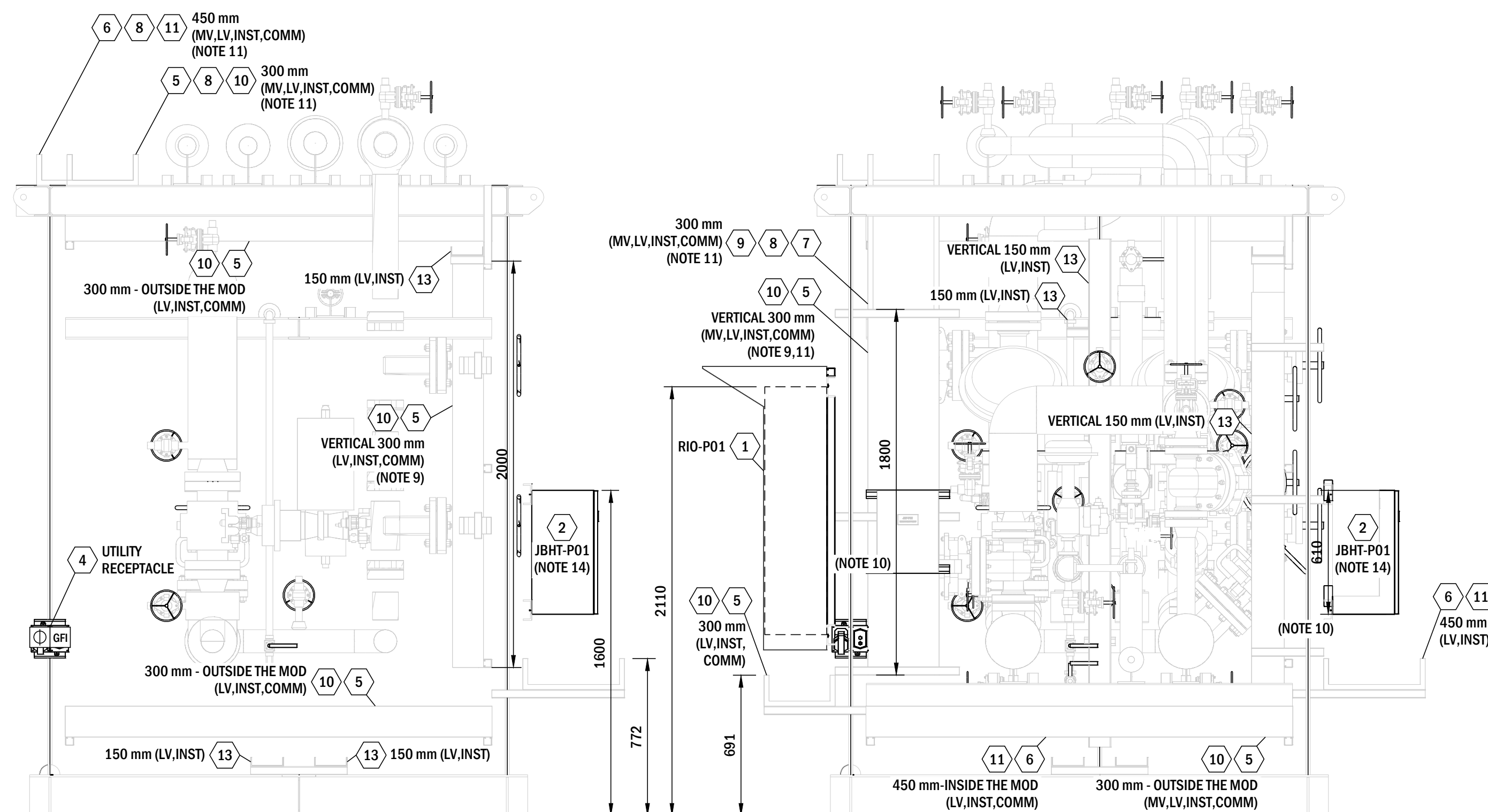
A SECTION VIEW ~ SCALE 1:20
