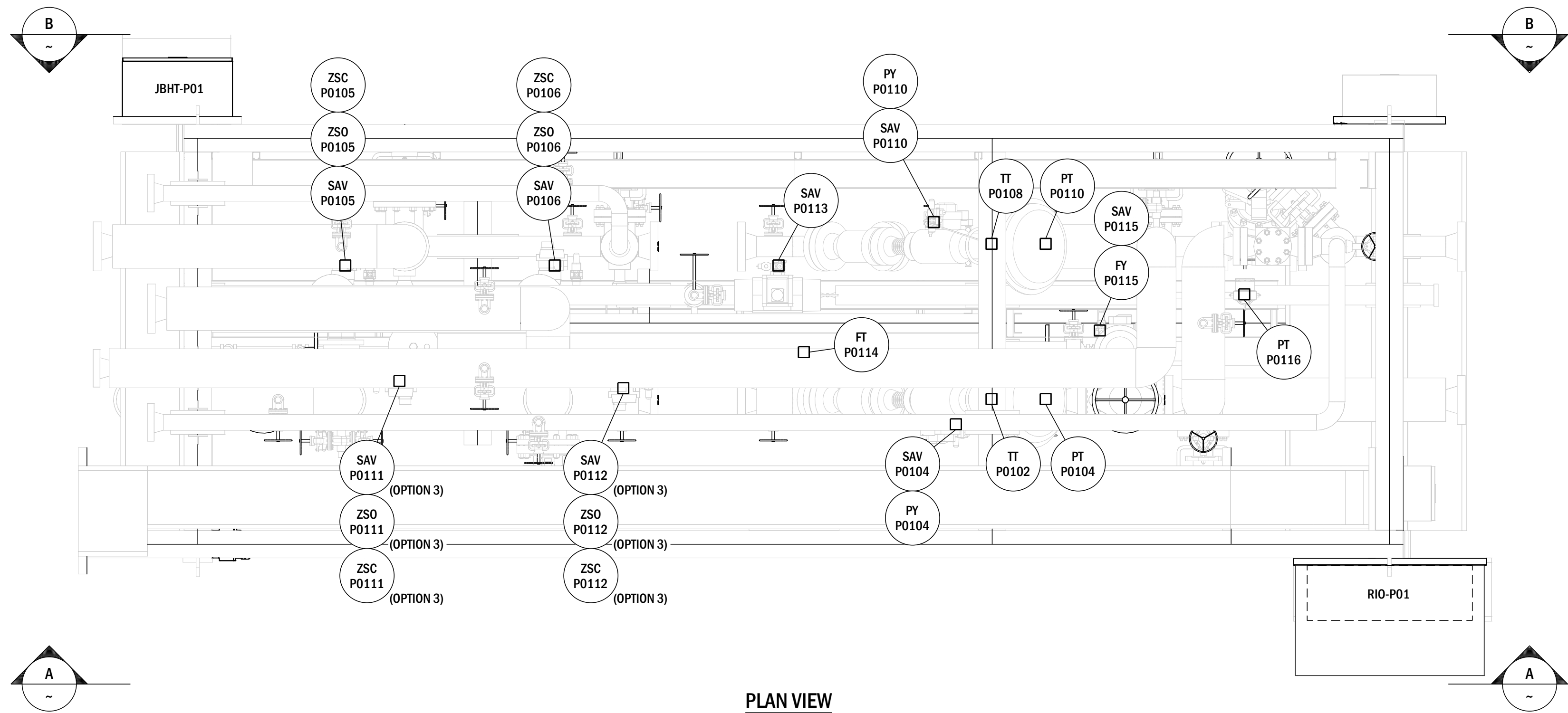
PLAN VIEW SCALE: 1:20
