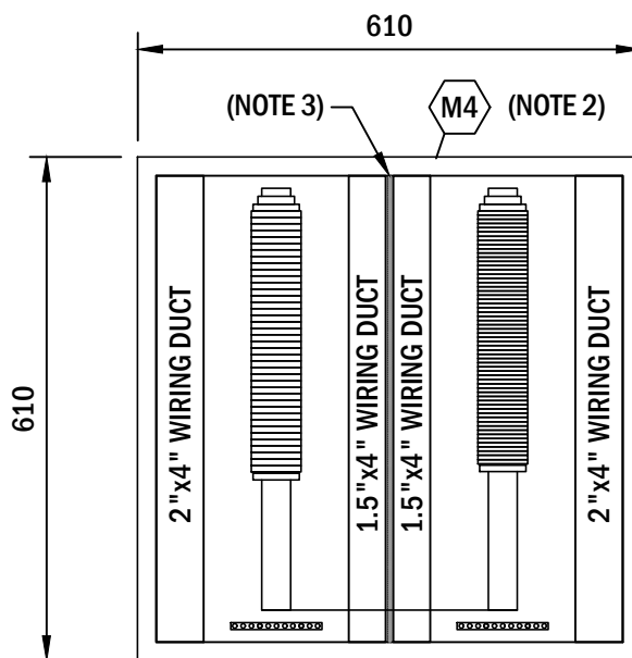
JUNCTION BOX DETAIL SCALE 1:10
