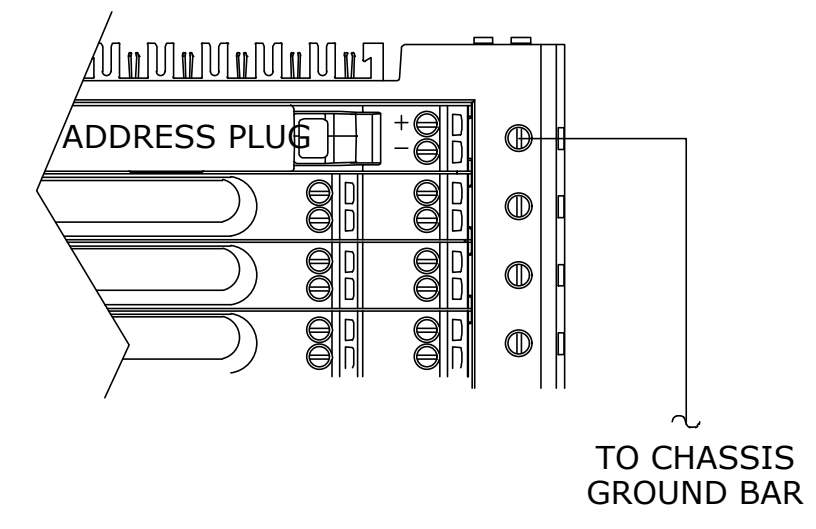
CIOC/CSLS BASEPLATE GROUND CONNECTION DETAIL
