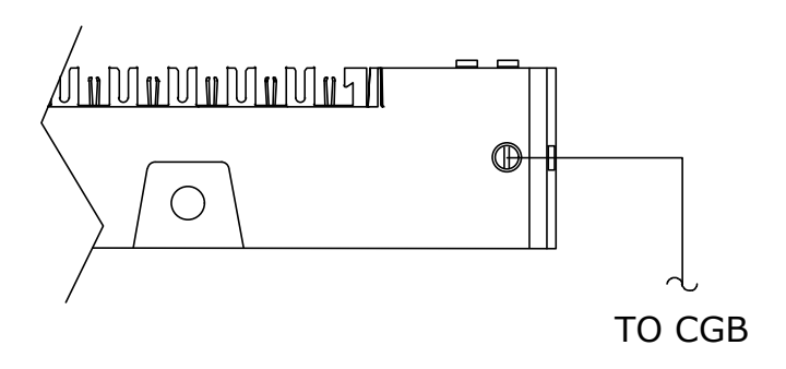
CIOC/CSLS BASEPLATE GROUND CONNECTION DETAIL
