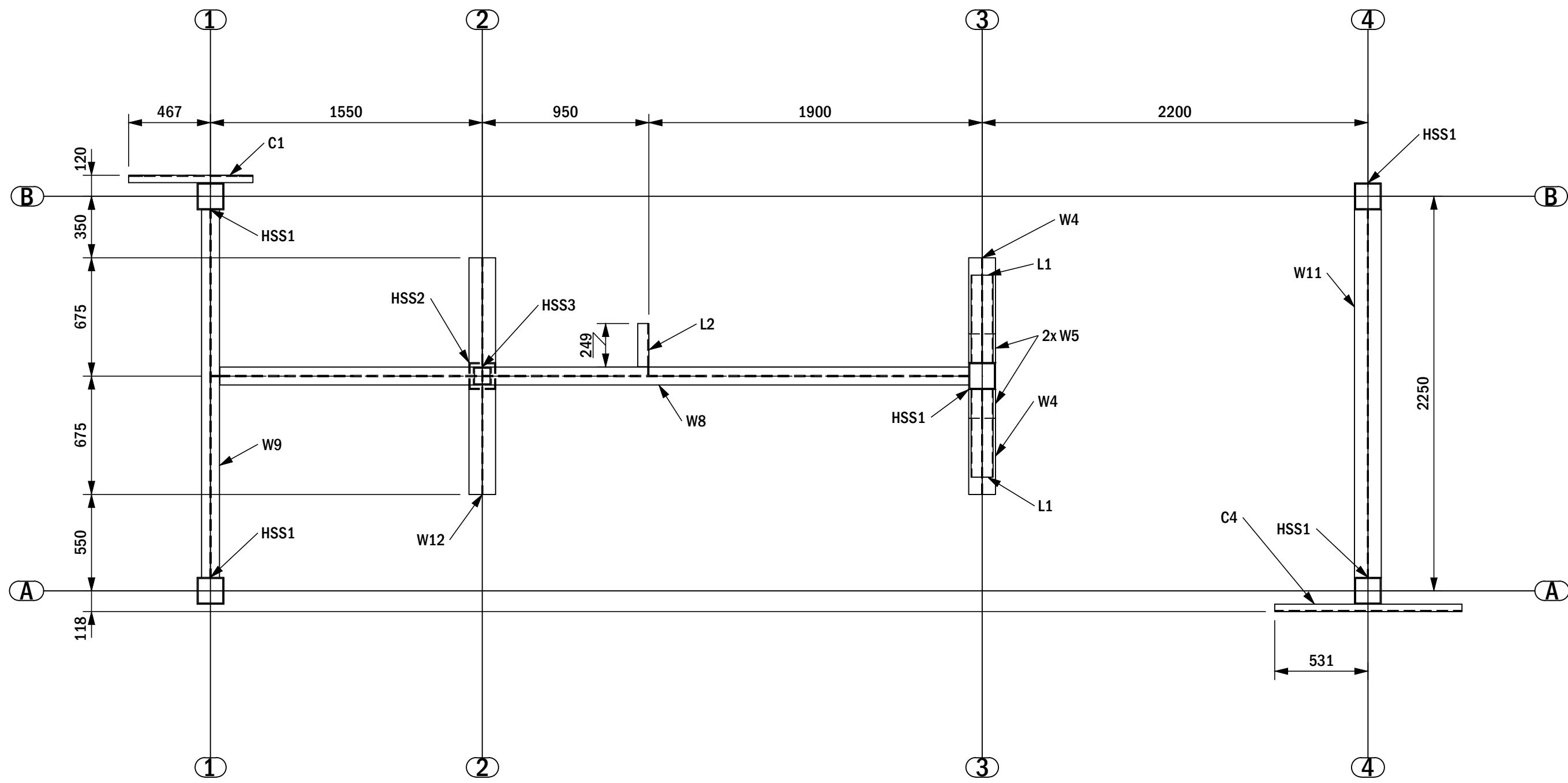
PLAN AT TOS EL. 2.250 SCALE 1:25
