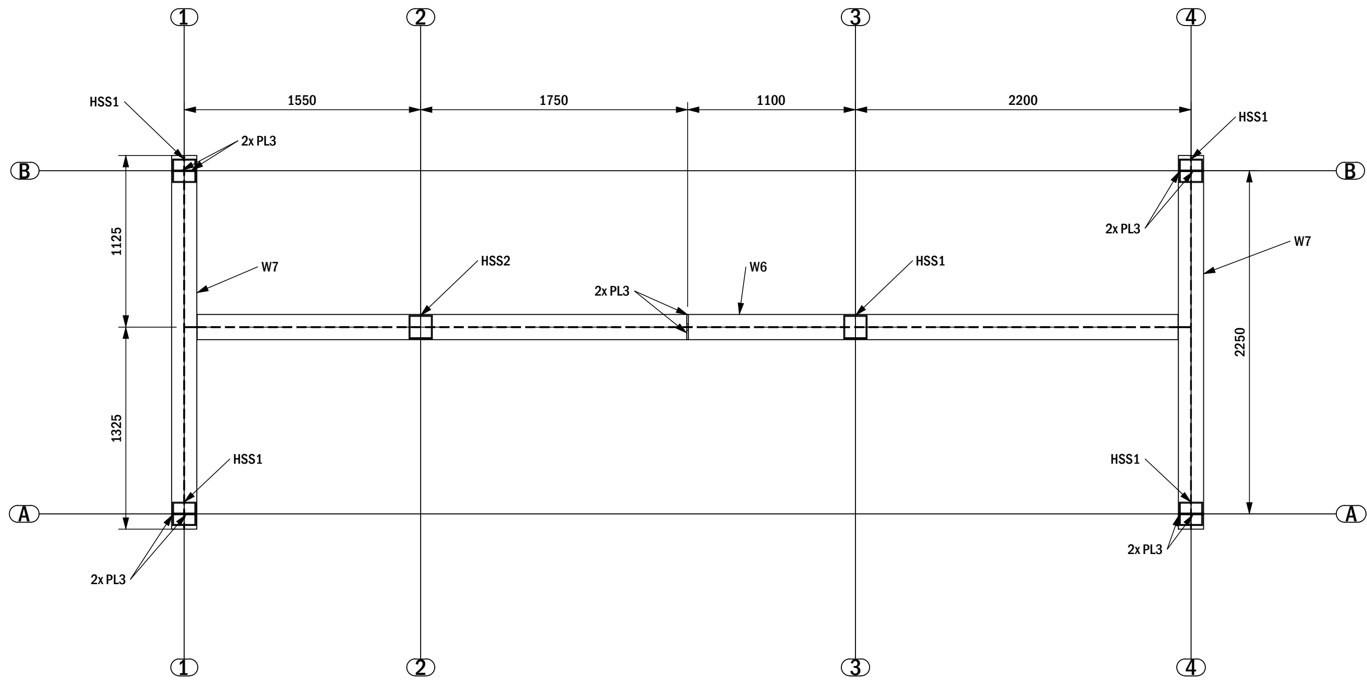
PLAN AT TOS EL. 0.000 SCALE 1:25
