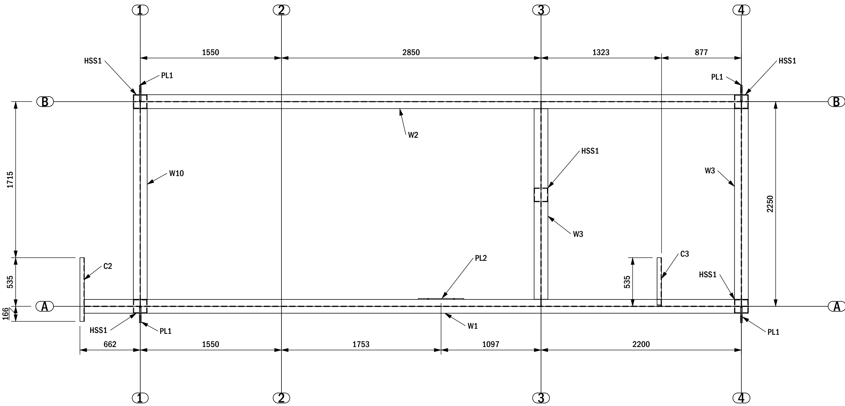
PLAN AT TOS EL. 2.900 SCALE 1:25
