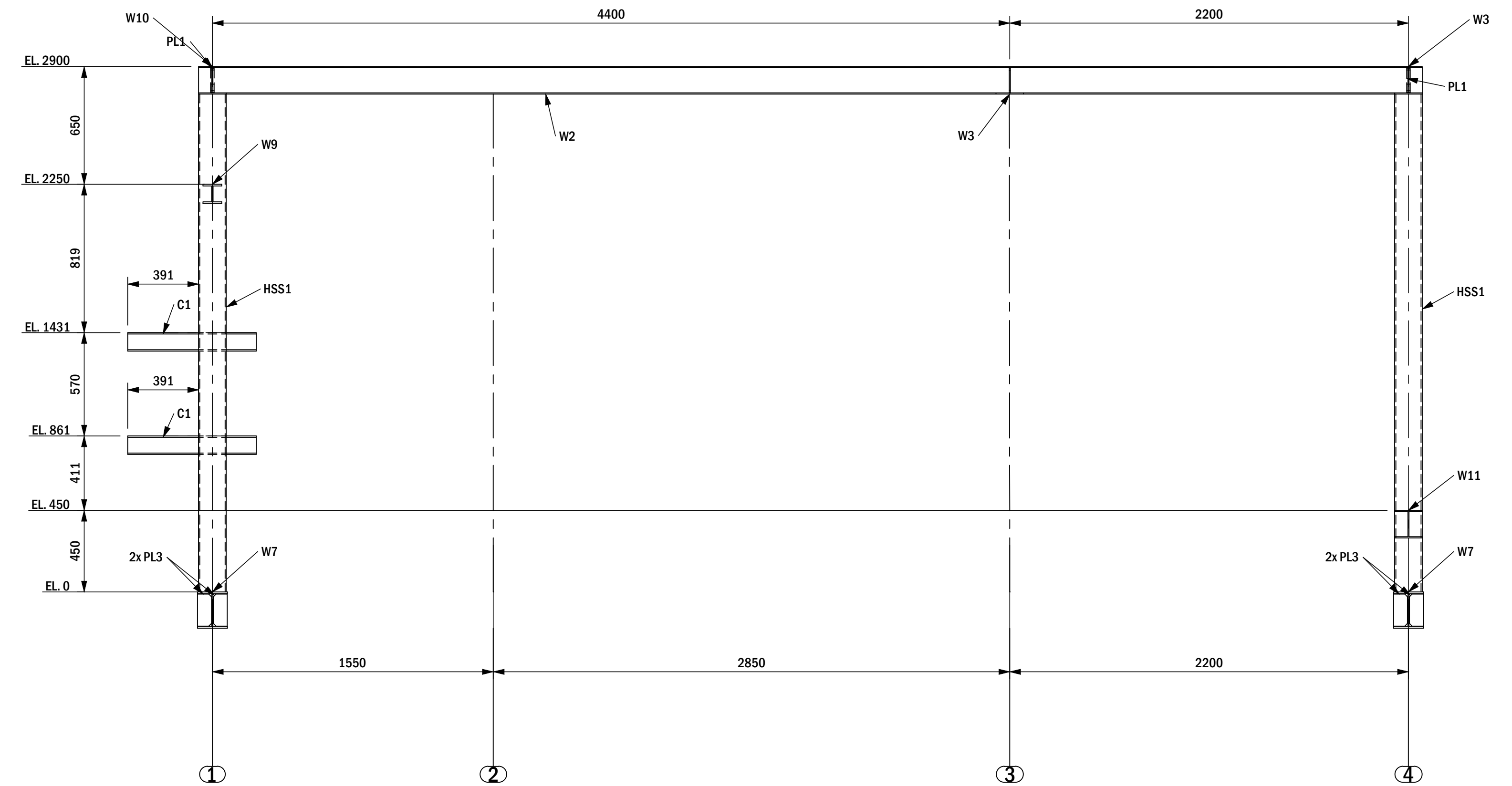
ELEVATION AT GRID LINE "A" SCALE 1:20
