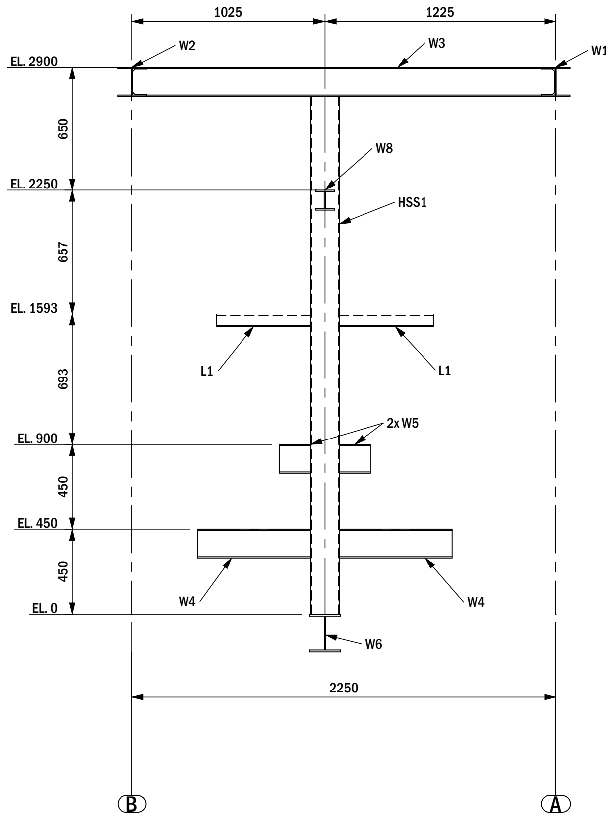
ELEVATION AT GRID LINE " 3 "
