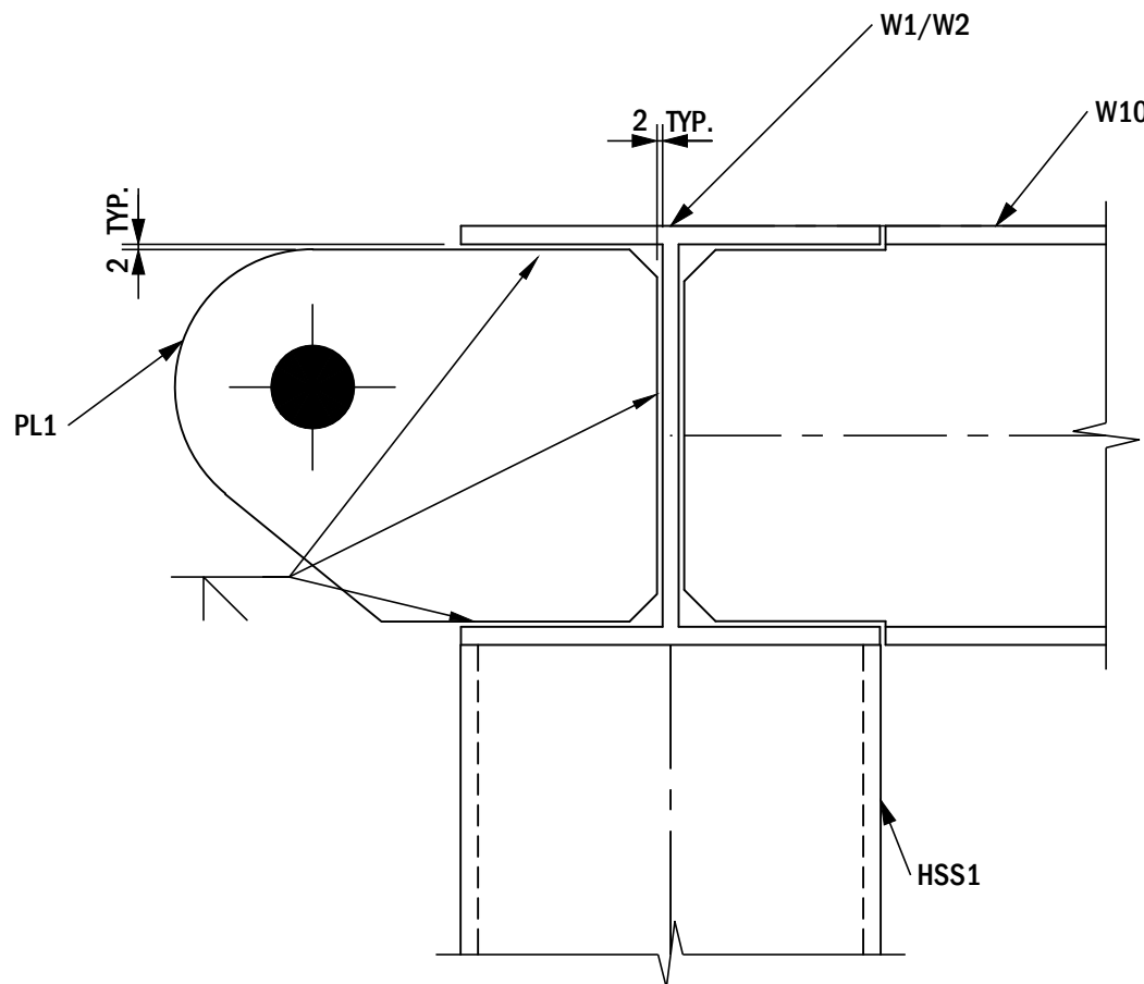
1 ~ SCALE 1:3 4 LOCATIONS
