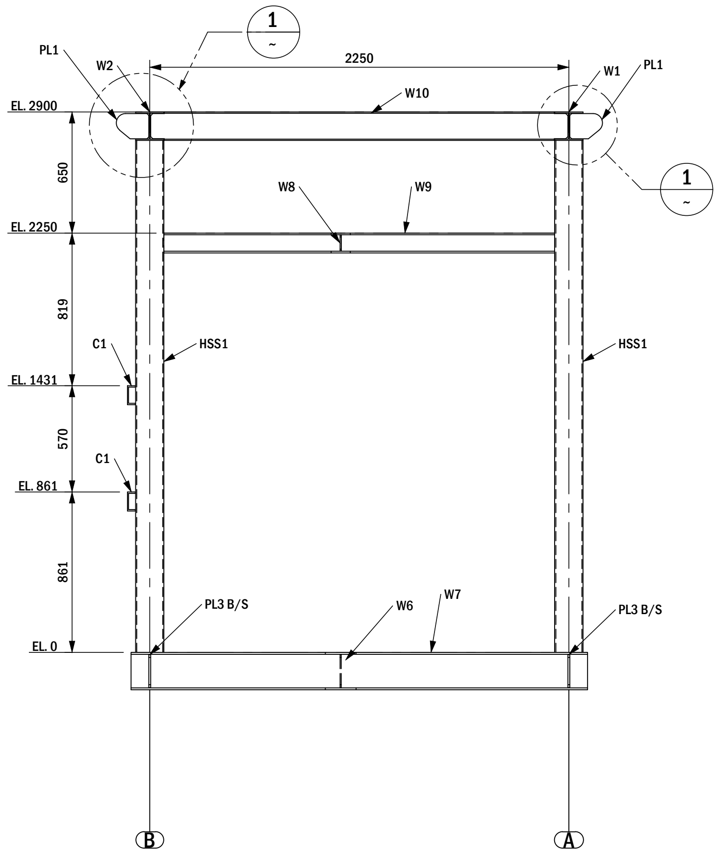
ELEVATION AT GRID LINE " 1 "
