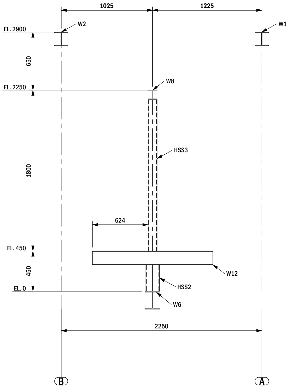
ELEVATION AT GRID LINE " 2 "
