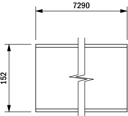
W1 SCALE 1:5 1 REQUIRED
