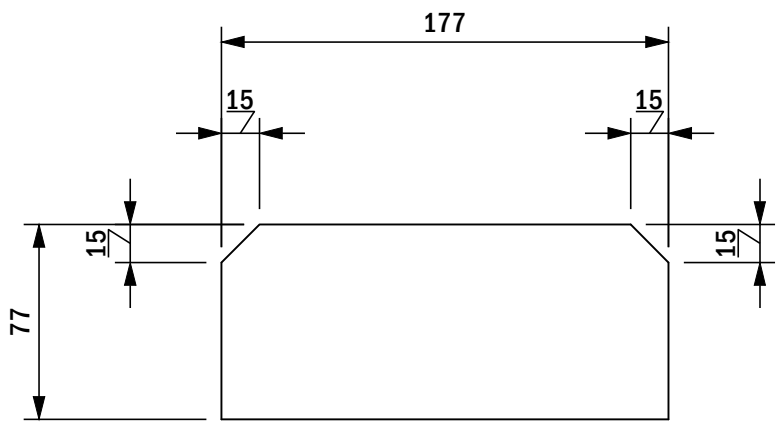
PL3 SCALE 1:3 10 REQUIRED
