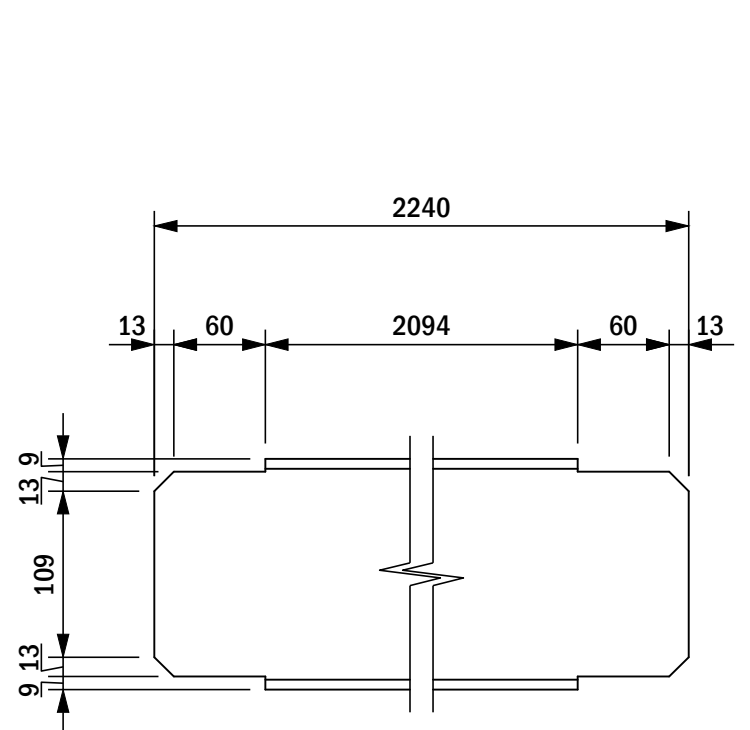
W3 SCALE 1:5 2 REQUIRED
