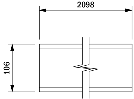
W9 SCALE 1:5 1 REQUIRED
