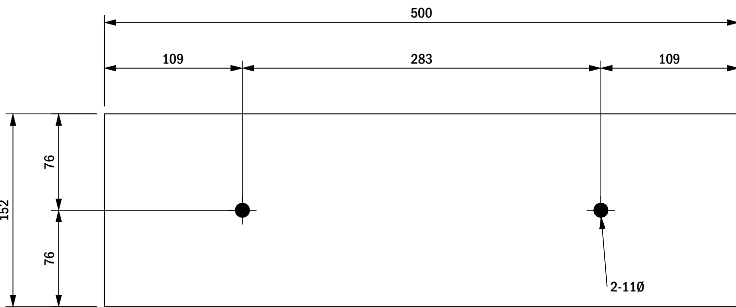
PL2 SCALE 1:3 1 REQUIRED
