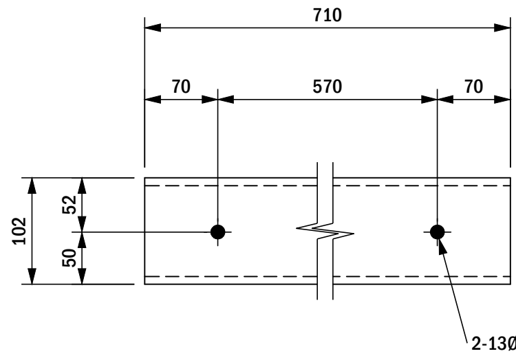
C1 SCALE 1:5 2 REQUIRED
