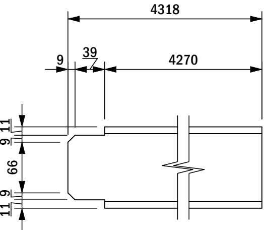
W8 SCALE 1:5 1 REQUIRED
