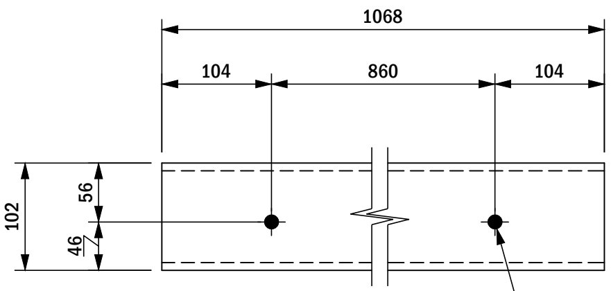
C4 SCALE 1:5 2 REQUIRED
