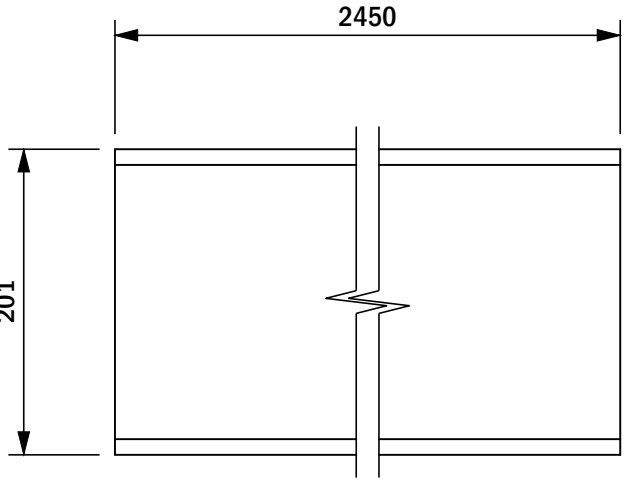
W7 SCALE 1:5 2 REQUIRED
