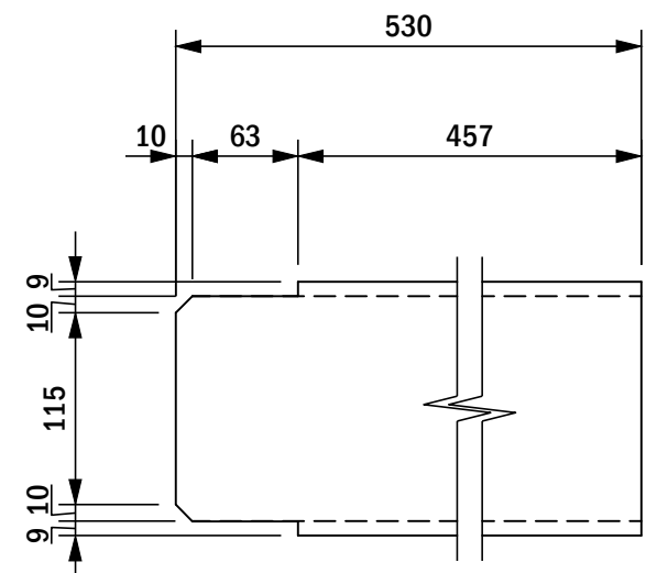
C3 SCALE 1:5 1 REQUIRED
