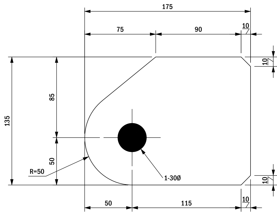
PL1 SCALE 1:2 4 REQUIRED
