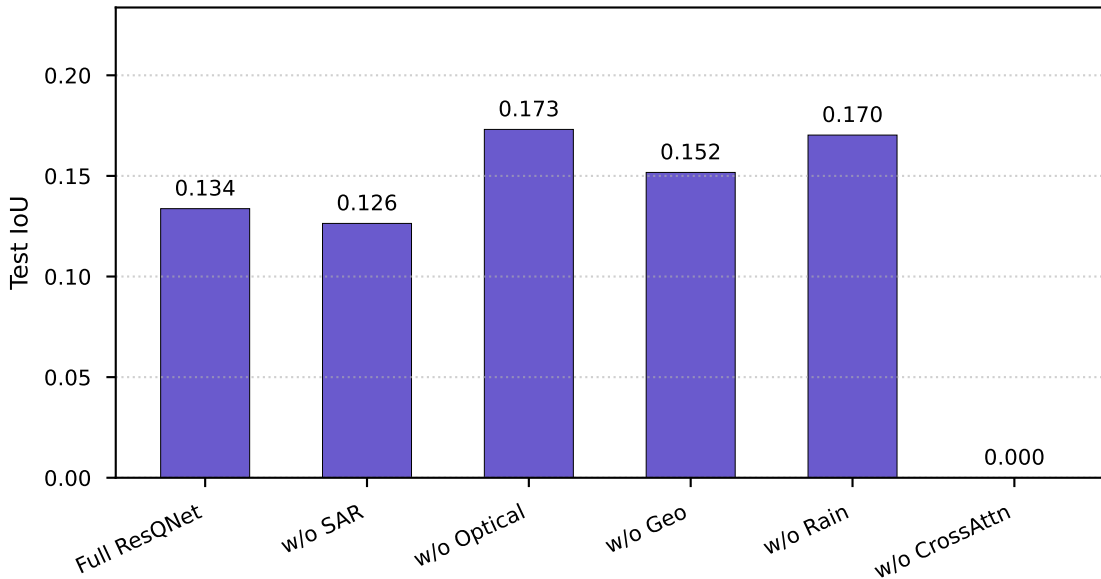
Ablation Study (Synthetic Smoke Benchmark)
