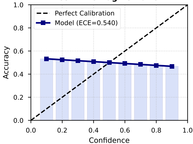
Test-Time Augmentation
