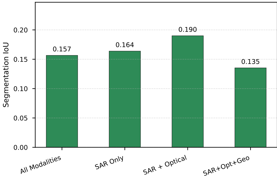
Robustness (Synthetic Smoke Benchmark)
