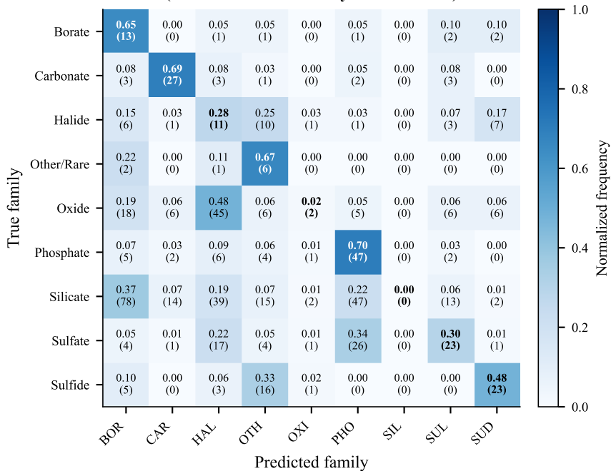
Normalized Confusion Matrix – RamanFormer1D (9-class Chemical Family Classification)
