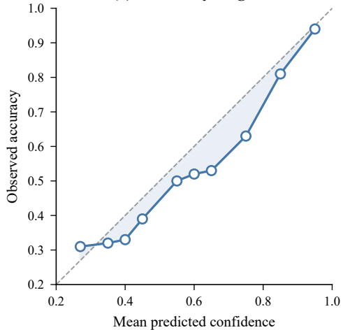
(a) Reliability diagram
