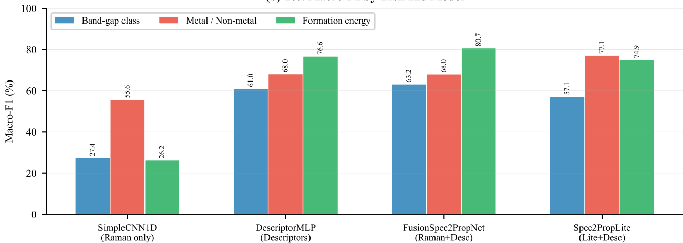
(b) Test Macro-F1 by Task and Model
