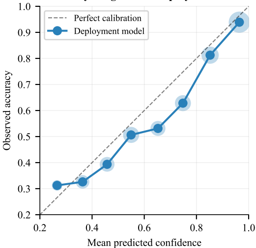
Reliability Diagram — Deployment Model
