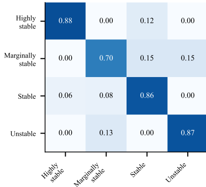
Formation Energy Classification (FusionSpec2PropNet)
