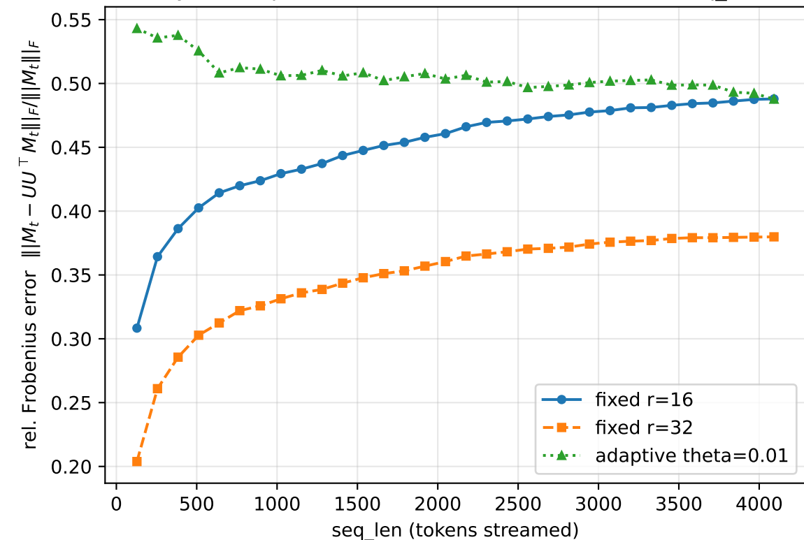
Layer-8 K (post-RoPE): reconstruction error vs. seq_len
