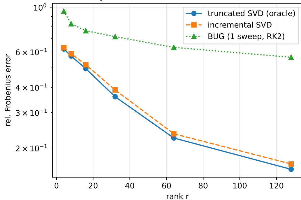
layer 15 reconstruction error vs. rank
