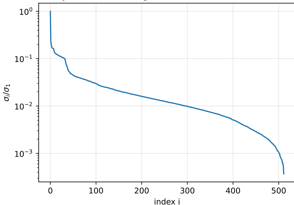
layer 8 K-cache singular values (no first-4 sinks)
