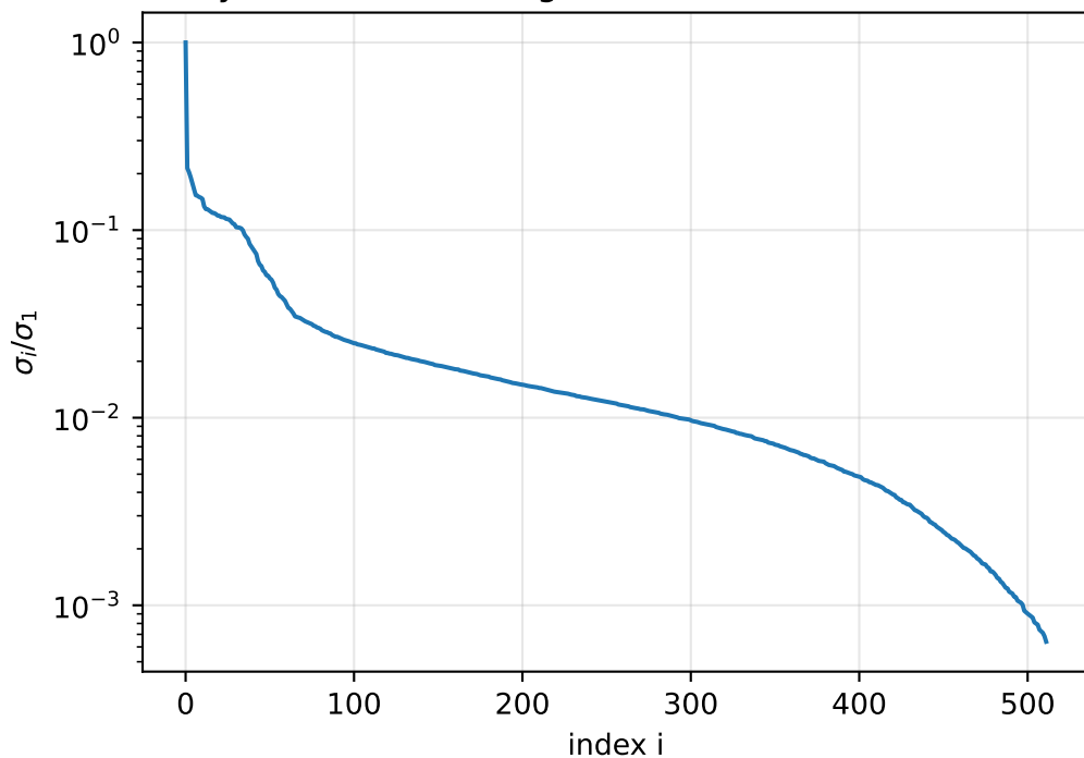
layer 15 K-cache singular values (no first-4 sinks)
