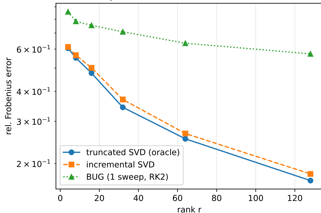
layer 8 reconstruction error vs. rank
