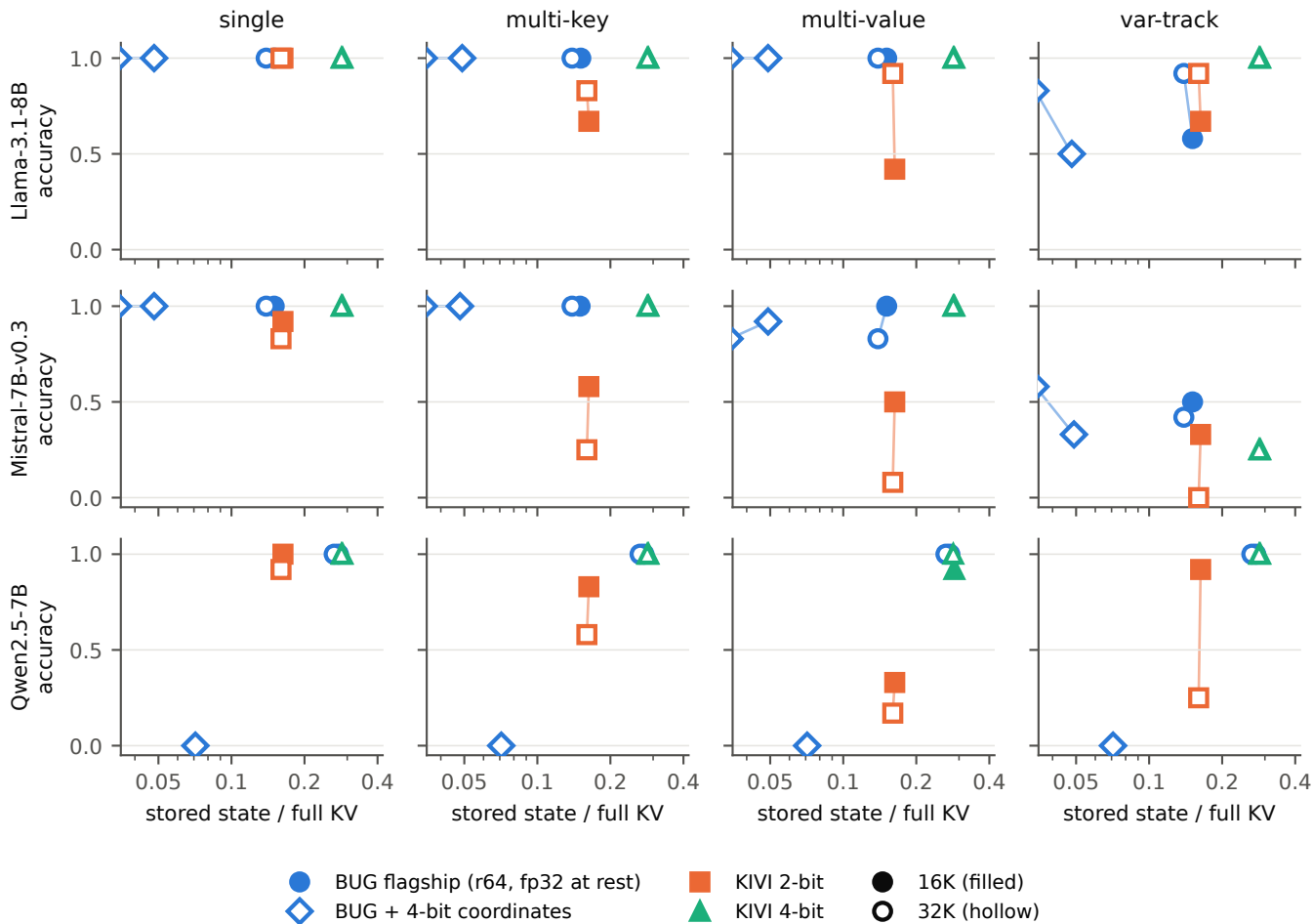
Retrieval vs stored bytes: flagship, its 4-bit-coordinate compose cell, and the fair KIVI baseline (n=12)
