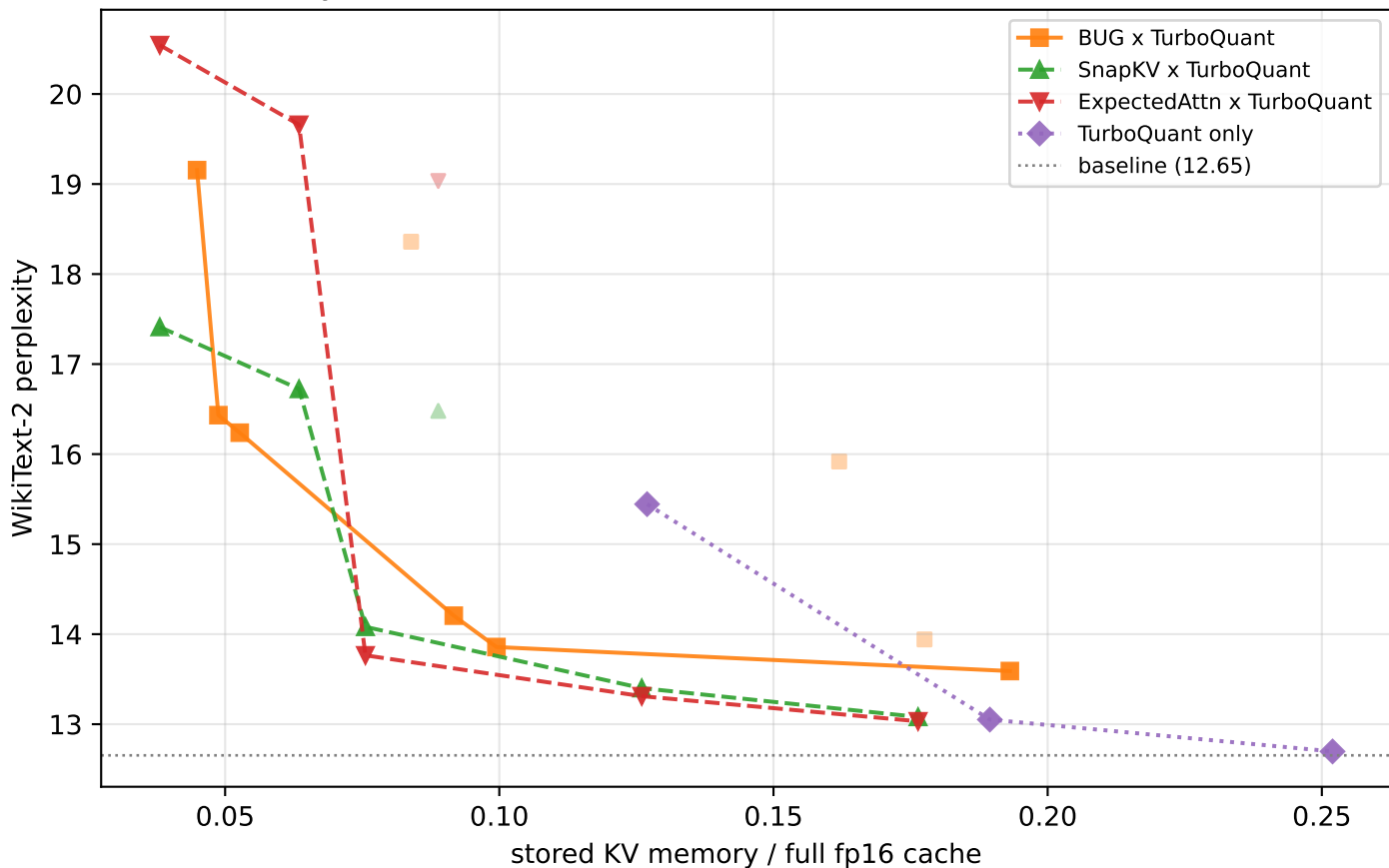
Fair: every mechanism x TurboQuant — Llama-3.2-1B-Instruct, ctx 1024
