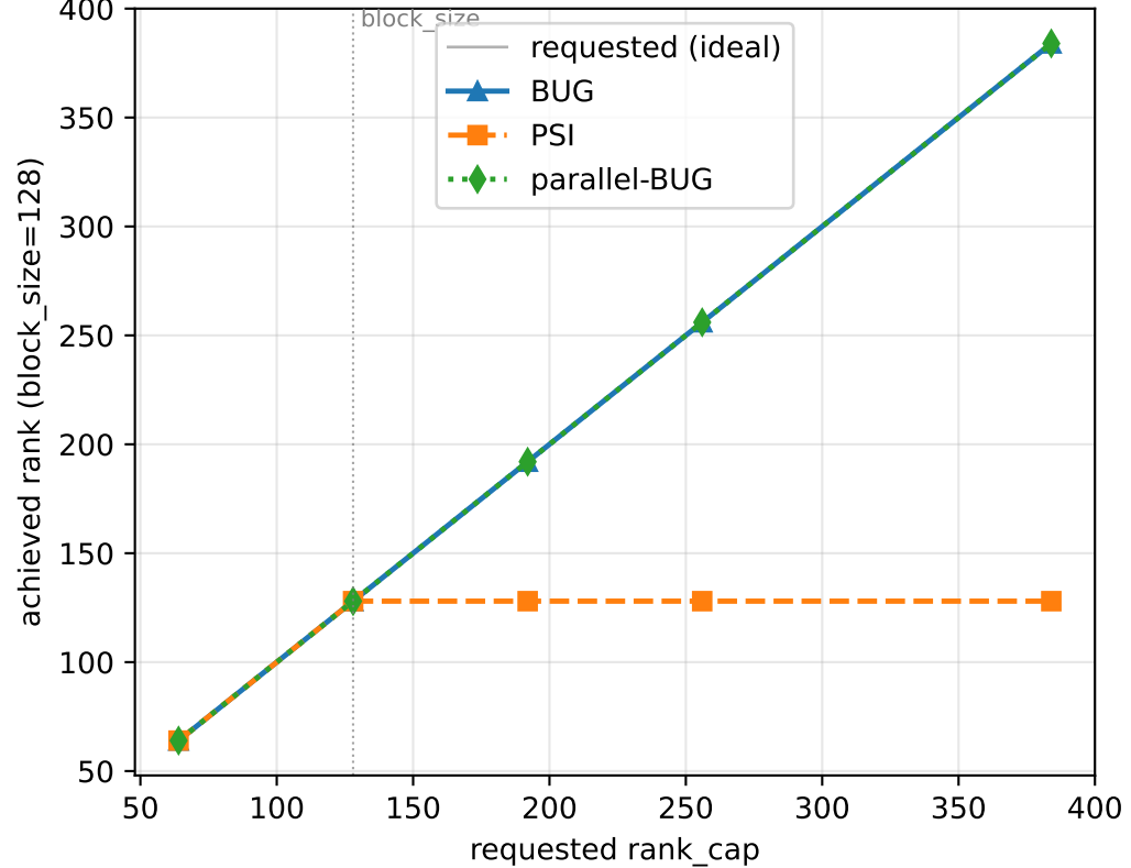
(b) streaming rank-adaptivity — PSI is fixed-rank
