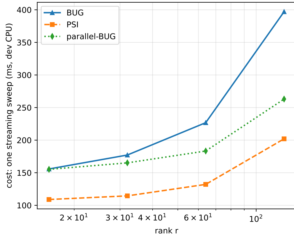
(c) per-sweep cost
