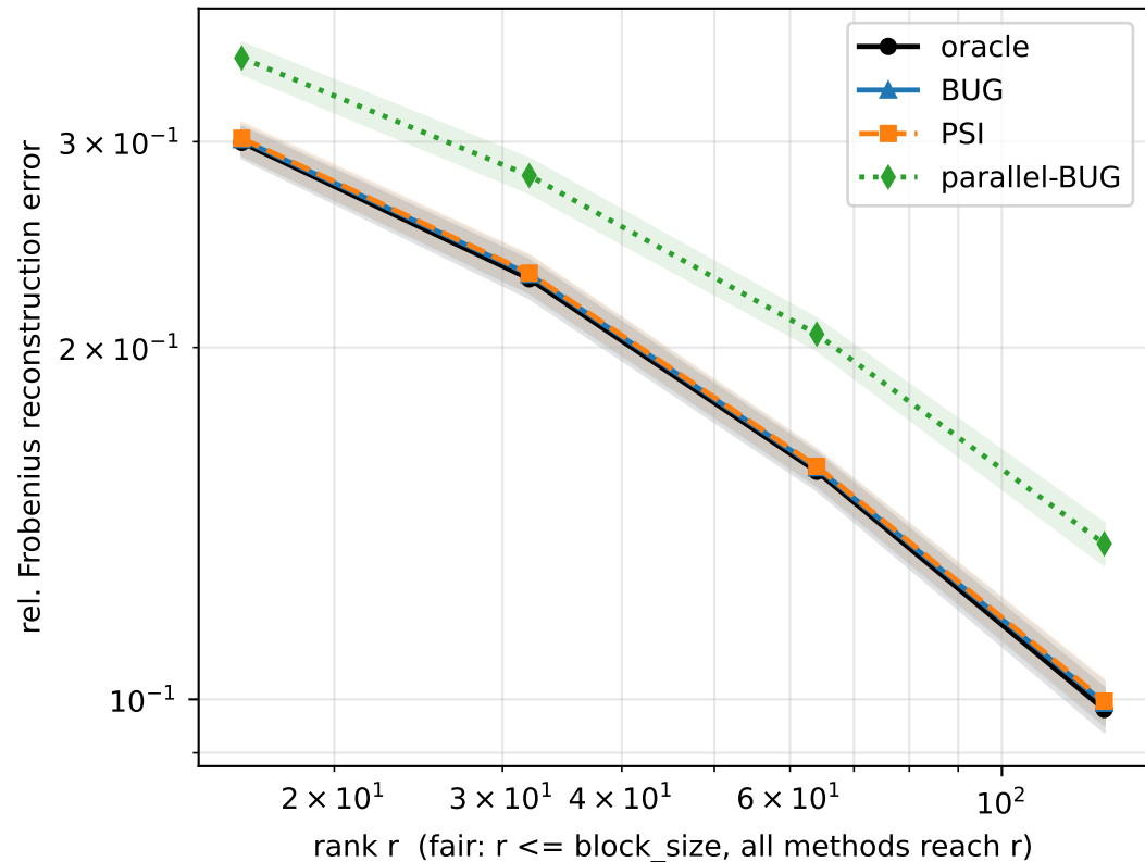
(a) accuracy vs rank — near-tie
